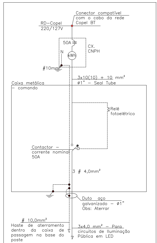
DIAGRAMA UNIFILAR
